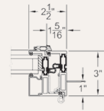
NAIL-ON JAMB AT HINGE
